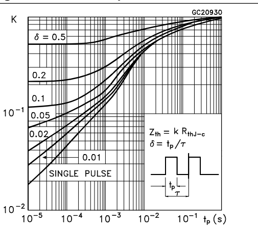
Figure 7. Thermal impedance for TO-220
