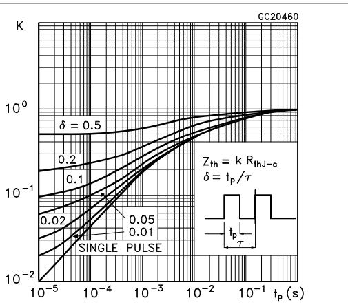
Figure 3. Thermal impedance for DPAK
